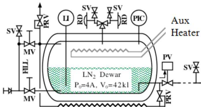
Fig. 3. P&ID of storage dewar
