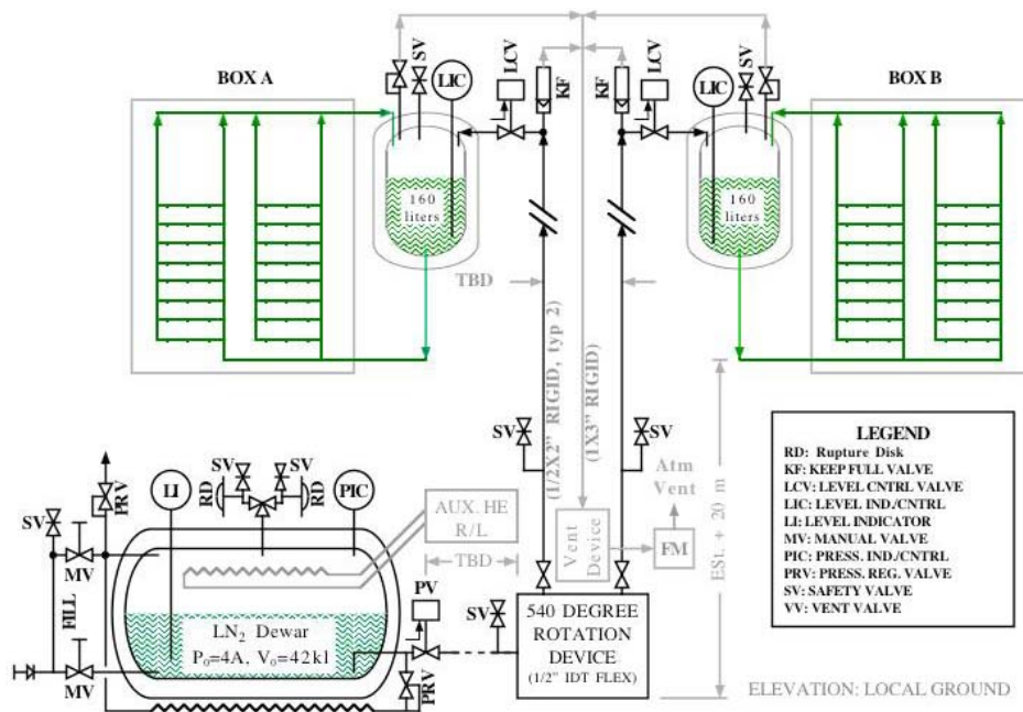
Fig. 1. VIRUS baseline cooling, simplified P&ID
