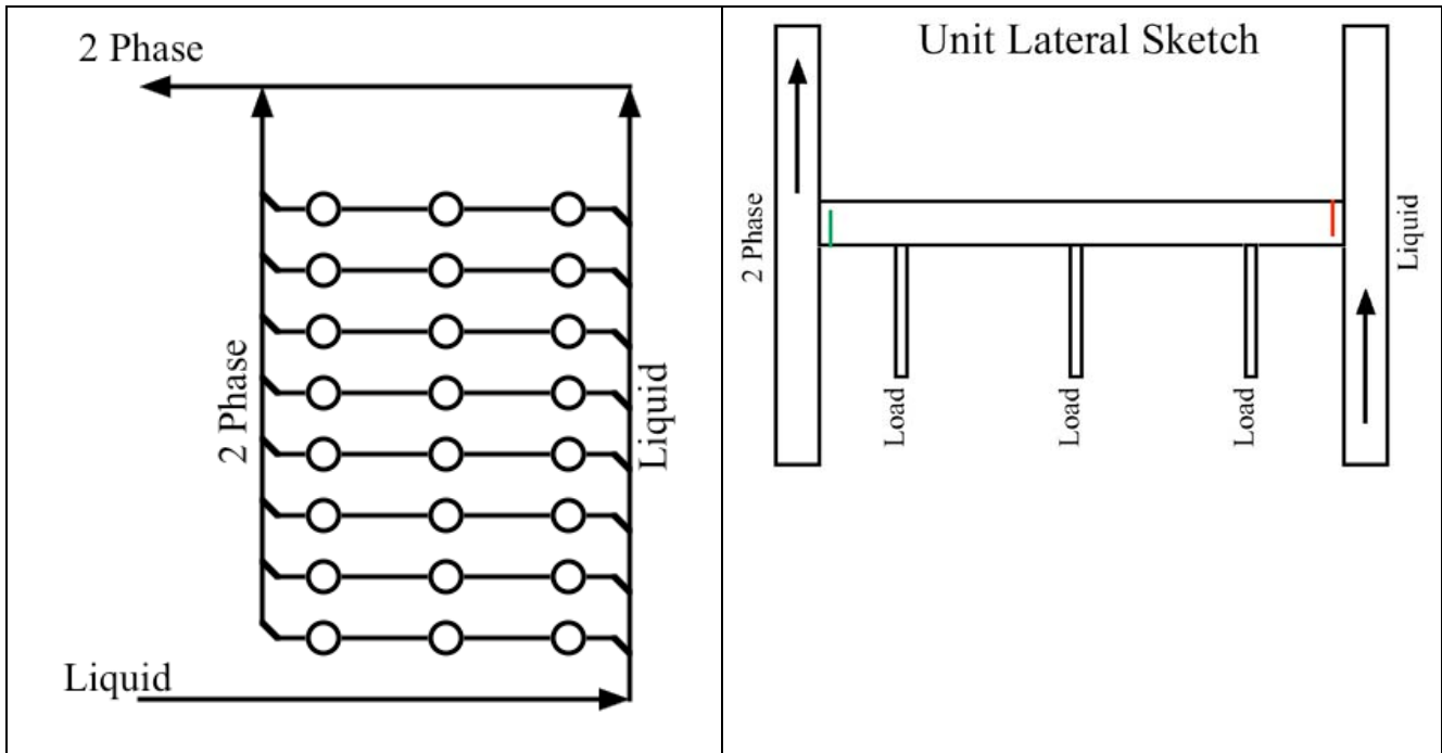
Fig. 5a. Manifold layout showing liquid and 2-phase risers
