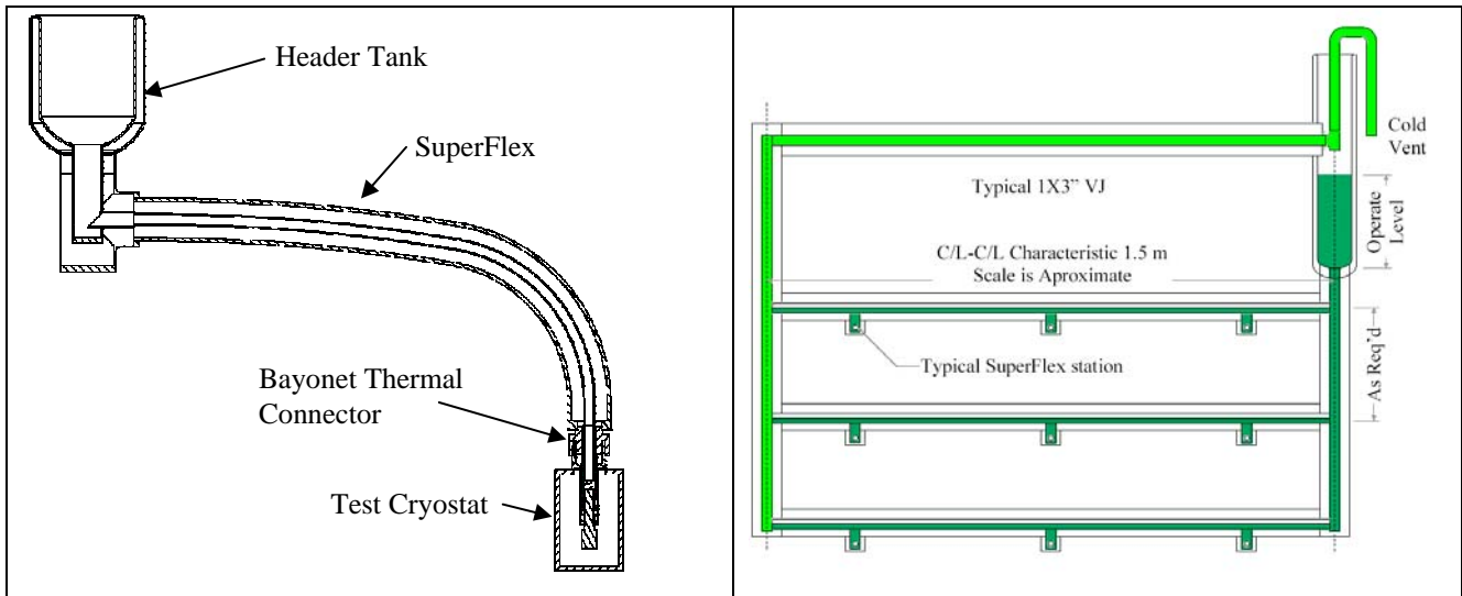
Fig. 9a. Liquid nitrogen header tank prototype to test performance of the SuperFlex, heat sink and thermal connector. 9b. Manifold power and flow test fixture to test performance of lateral manifolds and two-phase fluid removal.
